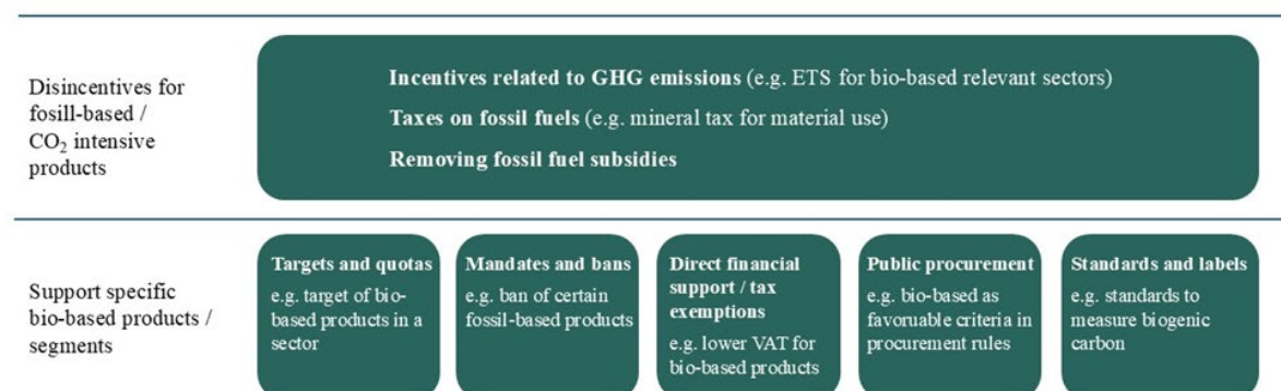
Figure 10: Demand-side policy instruments.
